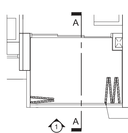
TYPICAL BALCONY SCREEN (OPEN)
