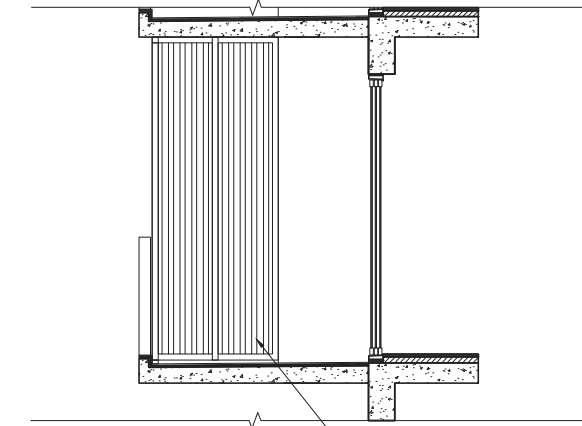
TYPICAL BALCONY SCREEN (CLOSED)
